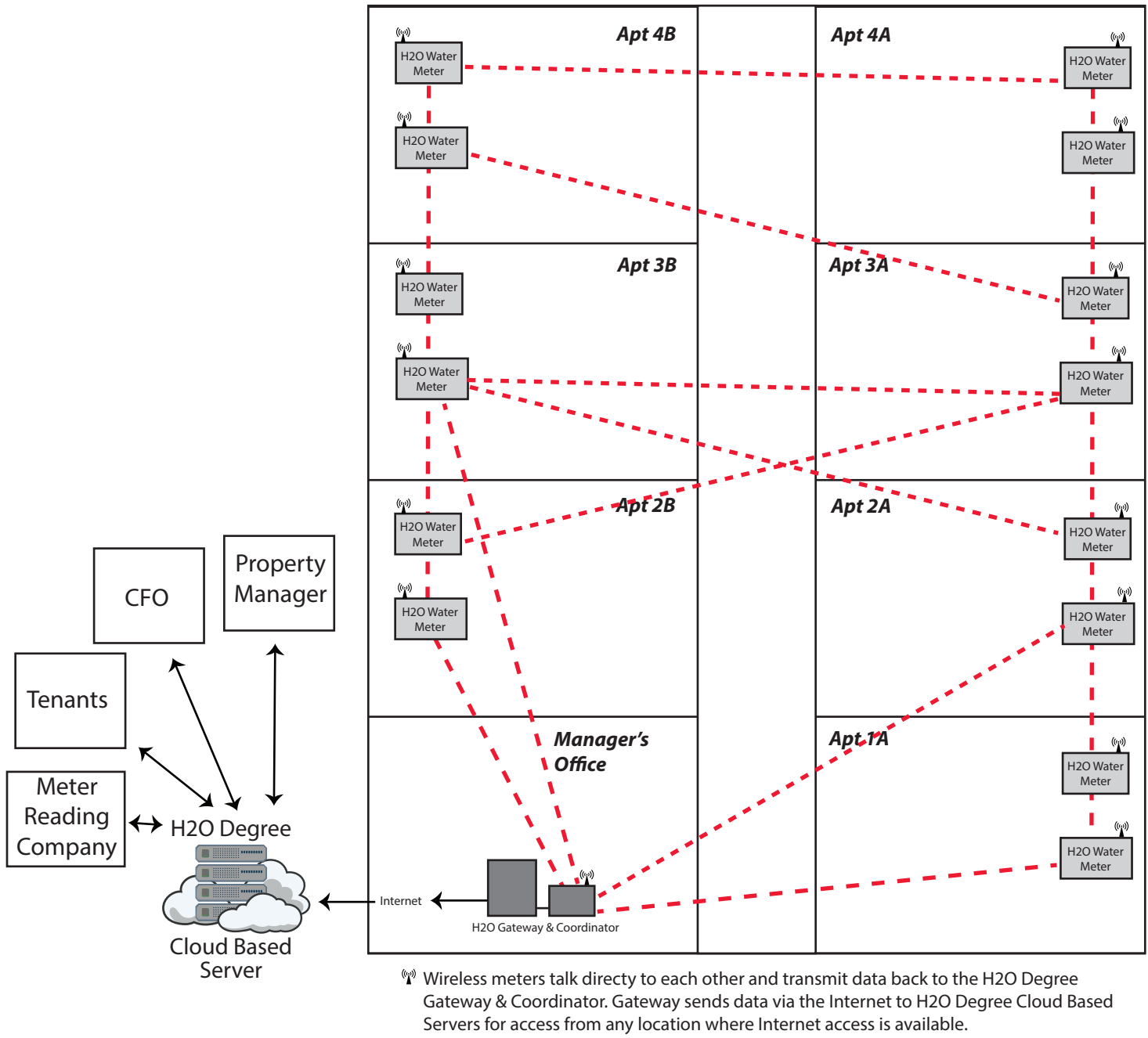
Line Powered Water Meter Building Configuration Diagram
